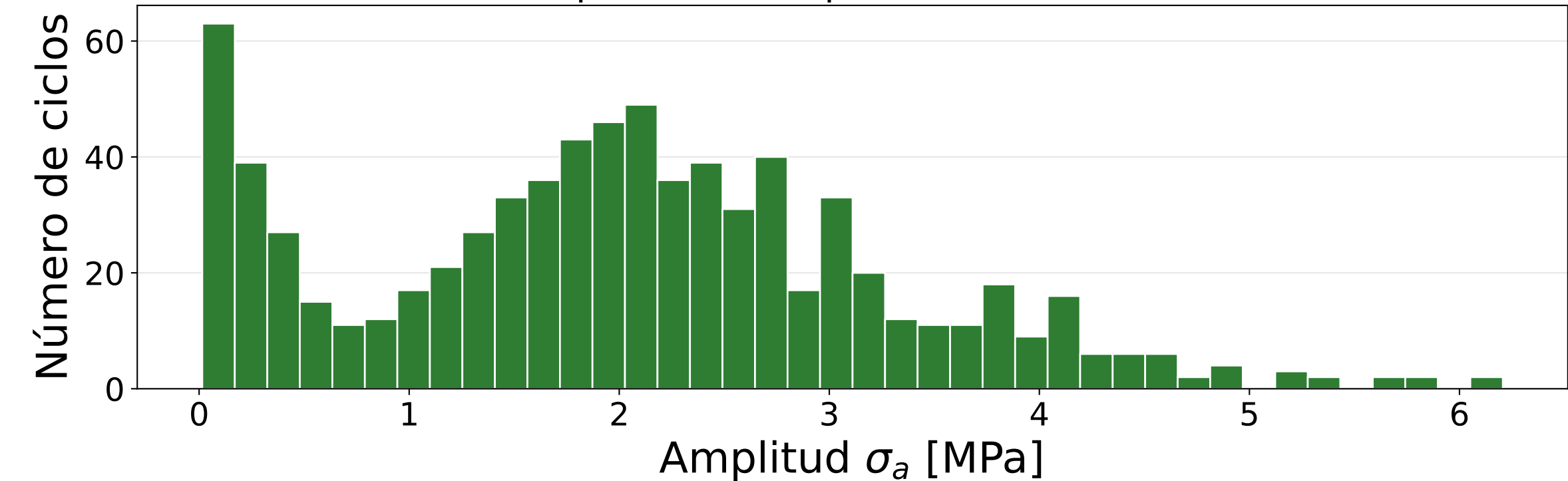
Espectro de amplitudes (Rainflow)
